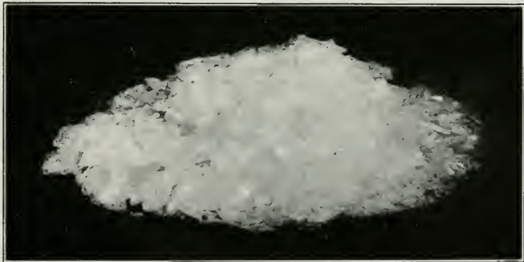
Fig. 35. Crystals of Silver Nitrate.
